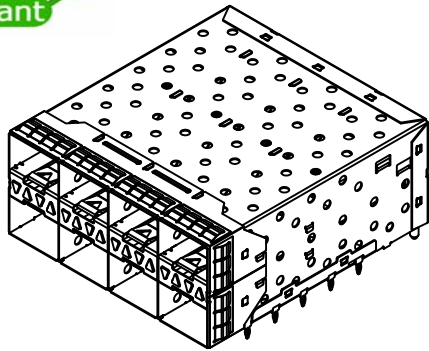
(4 LIGHT PIPE) E90-K410-4004
